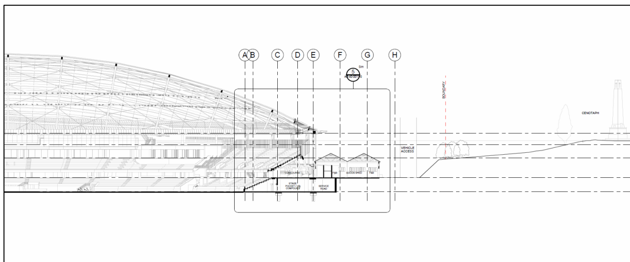
Figure 22: Partial site-section, north-south (source: COX Architects)
