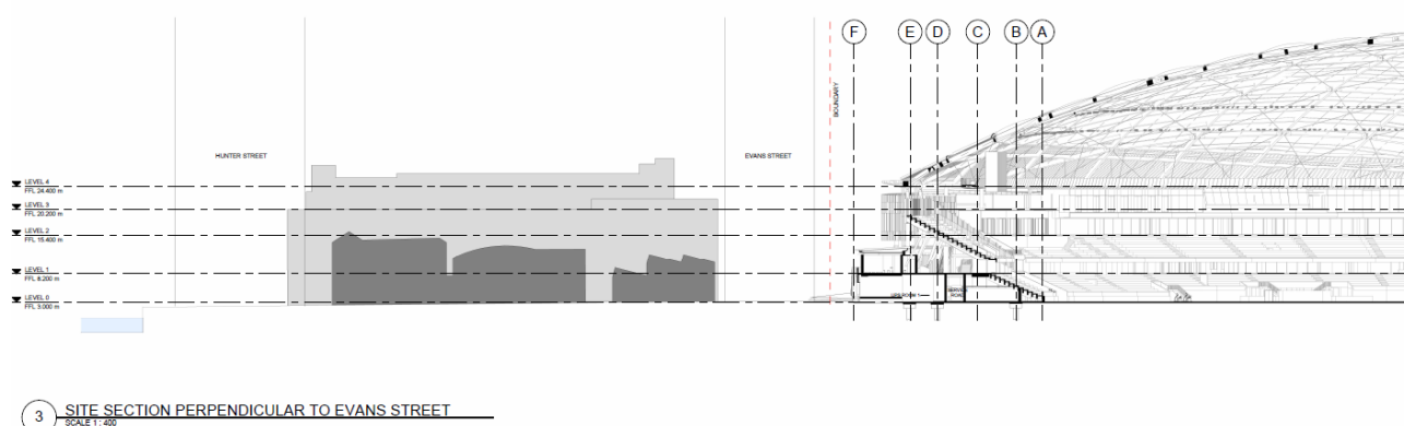
Figure 16: Site section along Evans Street (source: Appendix A - Architectural Documents, COX Architects).
