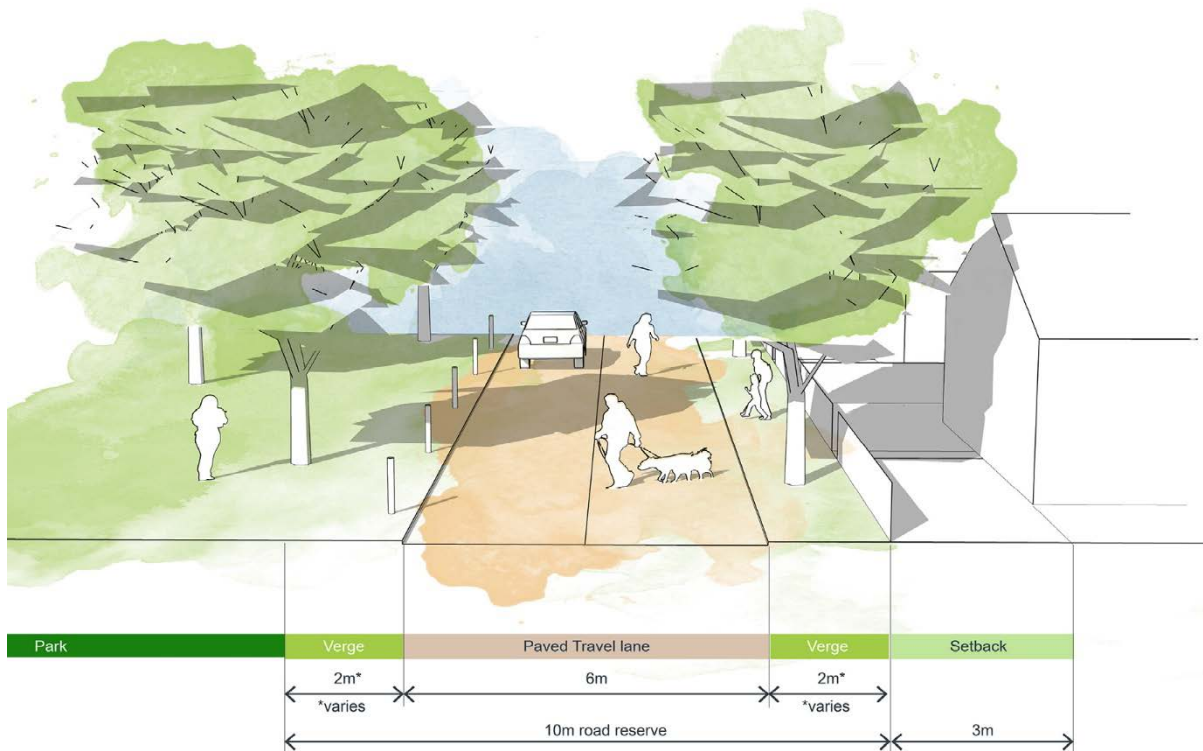
Figure DEV-S4.12 – Street typology for 10m wide shared zone reservation
