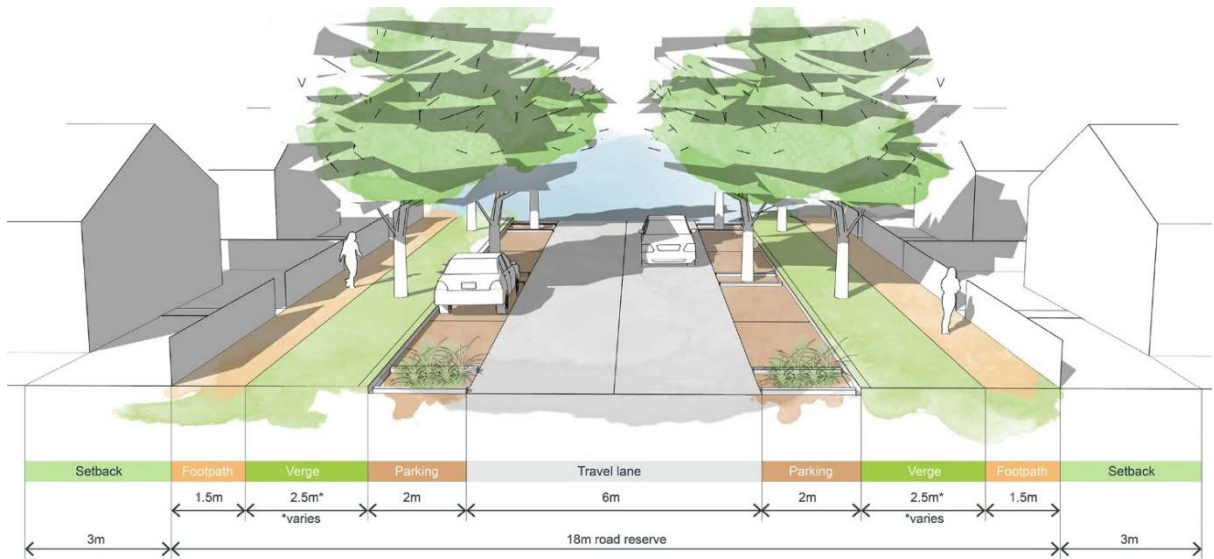
Figure DEV-S4.9 – Street typology for 18m wide reservation
