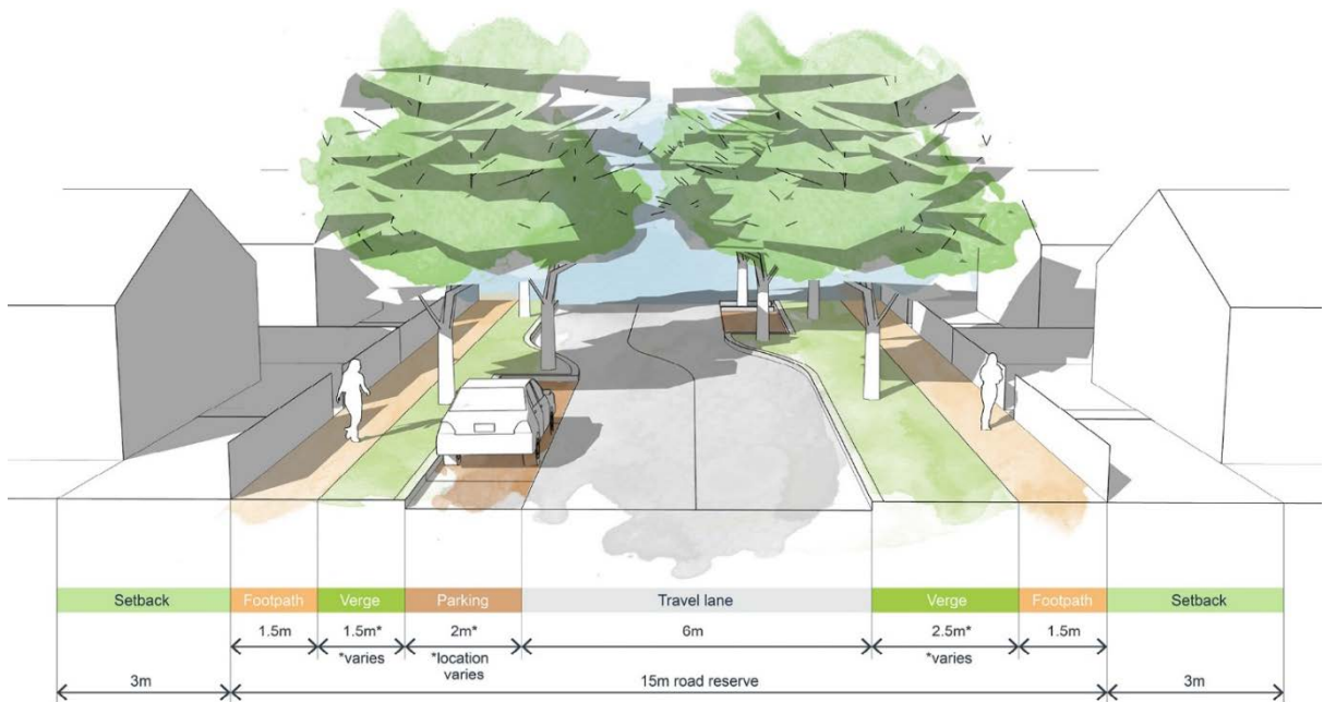
Figure DEV-S4.10 – Street typology for 15m wide reservation
