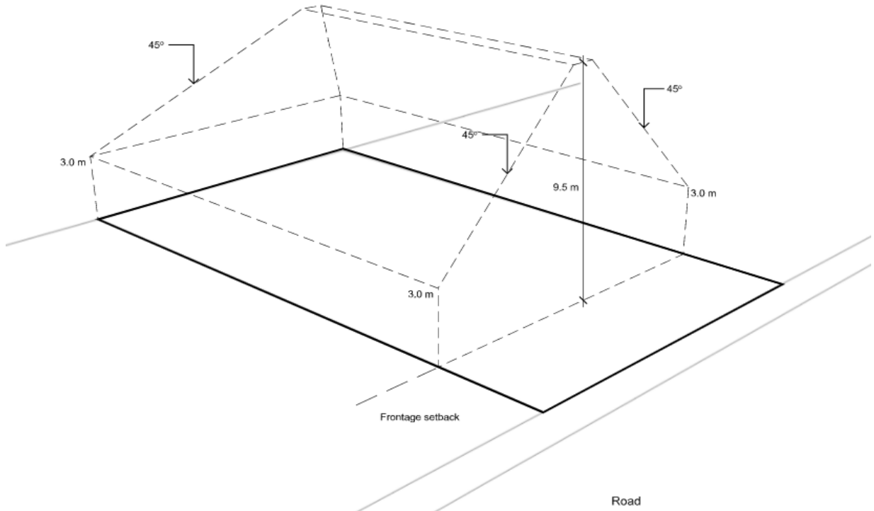
Figure DEV-S4.2 – Building envelope as required by clause DEV-S4.7.3
