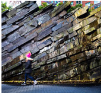
Dolerite formations
