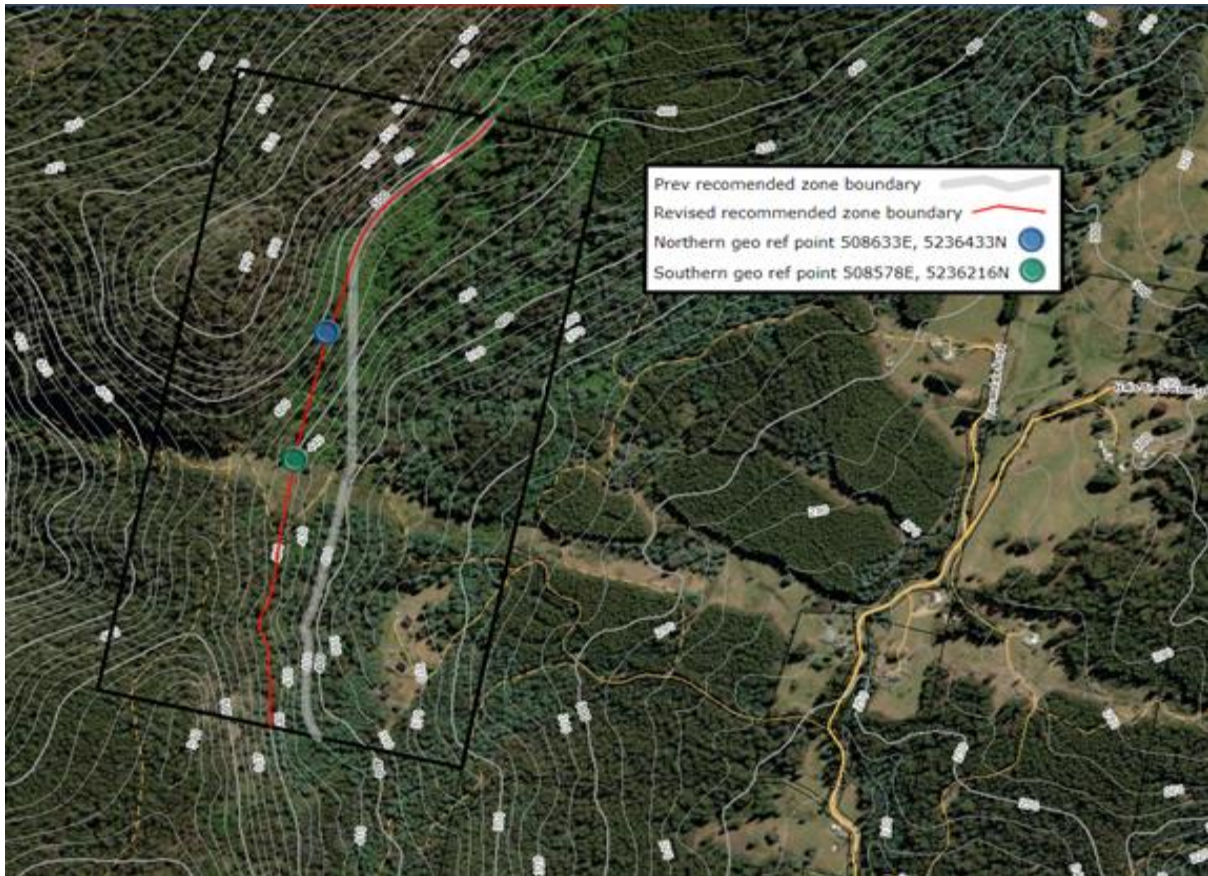
Figure 1 Split zoning diagram (Landscape Conservation Zone and Rural Zone) with 10m contours, cadastral parcels, road centrelines and ESRI imagery from www.thelist.tas.gov.au © the State of Tasmania
